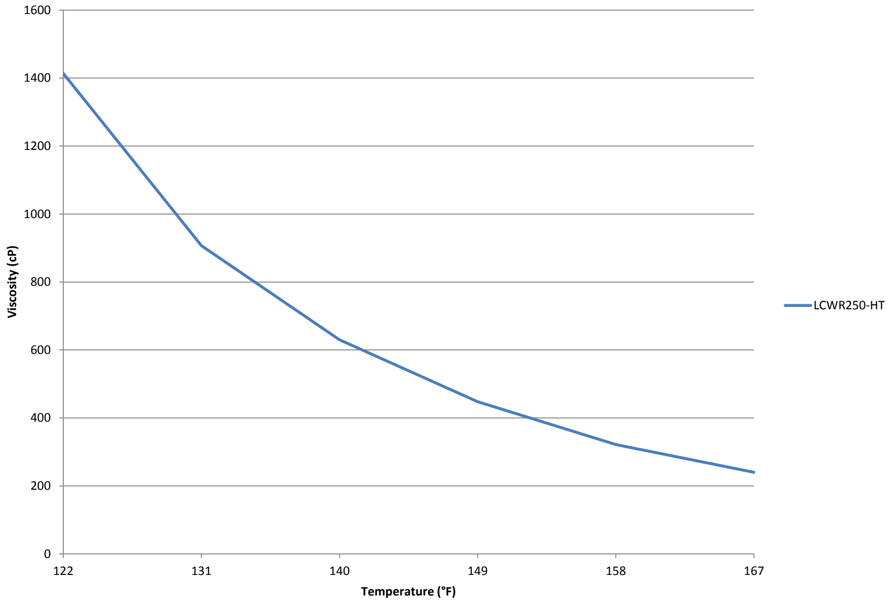
LCWR250-HT Viscosity Profile (120-170 °F)
